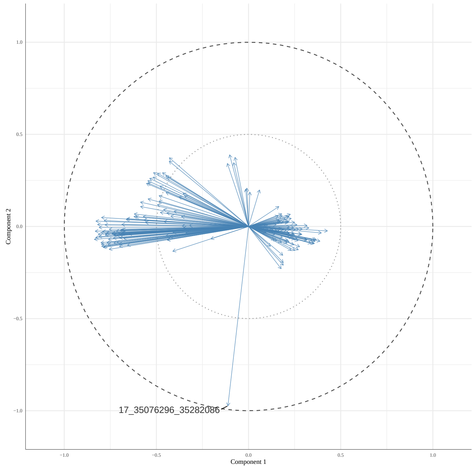
Correlation Circle Plot
